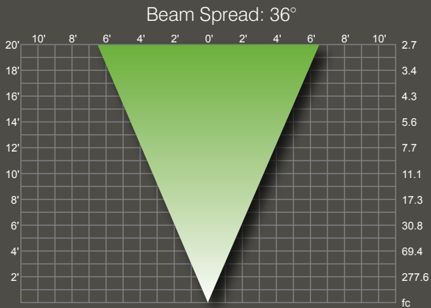
35W MR16: MR16FMW/L/AL
