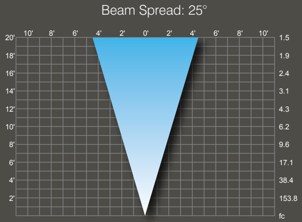
6W MR16: MR16/5M6WW25/LED
