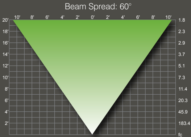
35W MR16: MR16WFL35/L/AL
