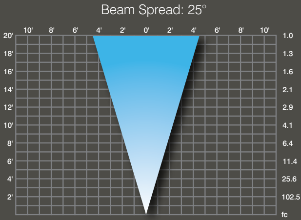
5W MR16: MR16/M5WW25/LED
