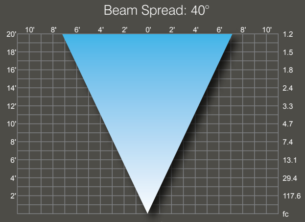
6W MR16: MR16/5M6WW40/LED
