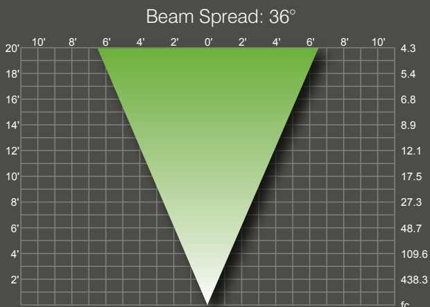
50W MR16: MR16EXN/L/AL
