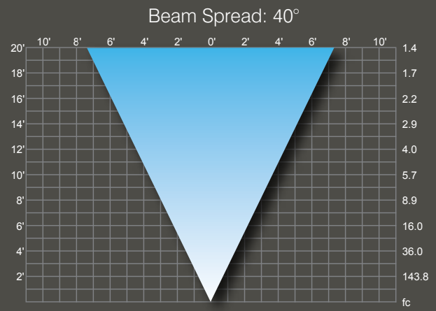
9W PAR36: PAR36/5WW/WFL/LED
