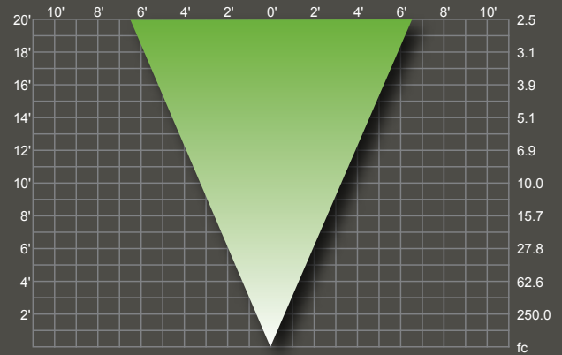
26W MR16: MR16FL35/L/26HX
