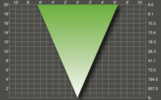
57W MR16: MR16FL75/L/57HX
