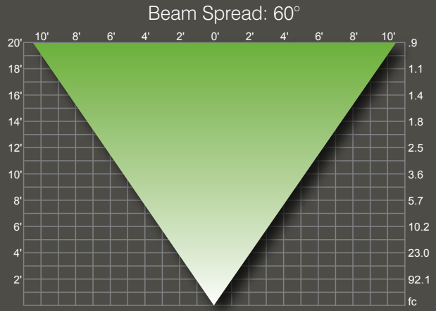
20W MR16: MR16WFL20/L/AL
