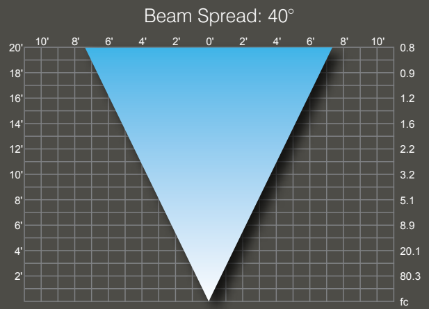
5W PAR36: PAR36/5WW/WFL/LED
