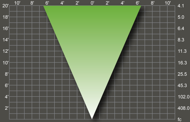
37W MR16: MR16FL50/L/37HX
