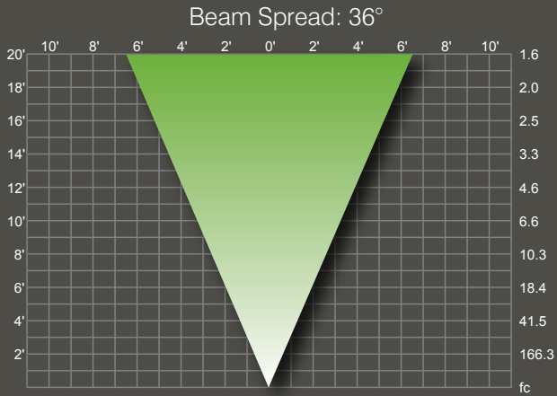
20W MR16: MR16BAB/L/AL
