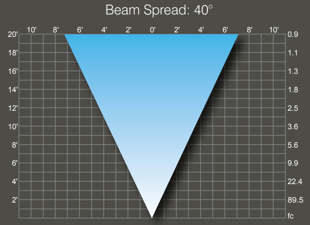
5W MR16: MR16/M5WW40/LED
